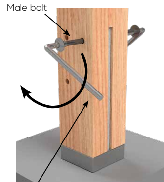
T50 Star Drive Wrench
